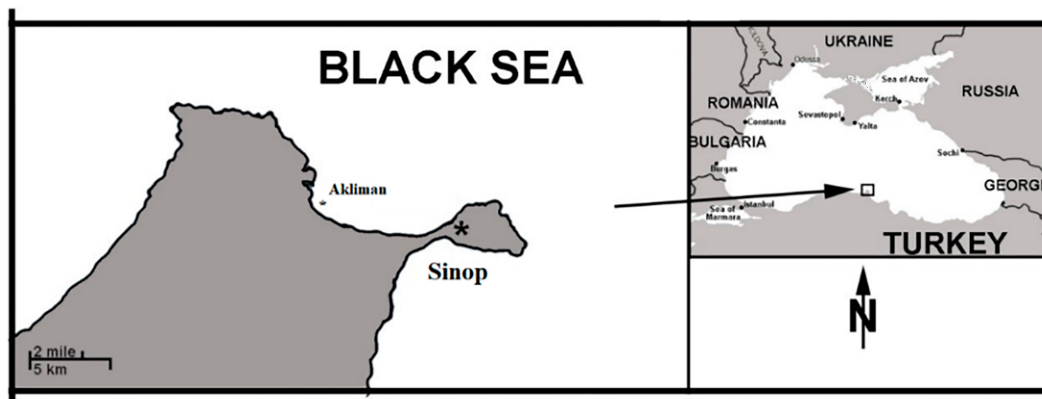
Fig. 2. Sampling area
