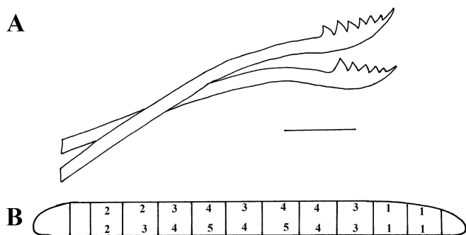
Fig. 2. A – chaetae of observed specimen Ctenodrilus serratus , scale bar 10 μm; B – schematic representation of the number of chaetae in chaetigers of C. serratus in notopodia (upper row) and neuropodia (lower row)
