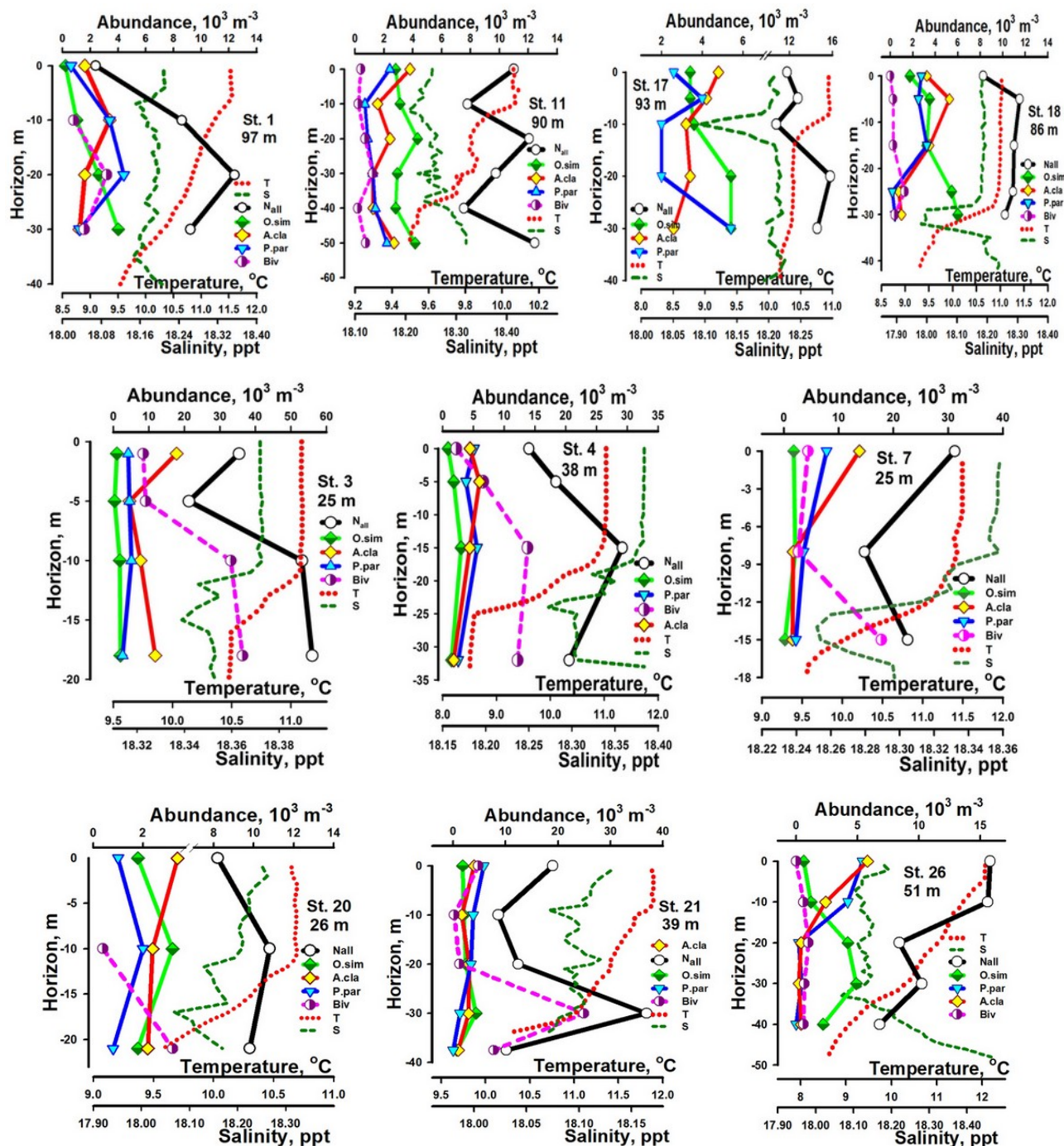
Fig. 2. Vertical distribution of water temperature (T), salinity (S), abundance of total metazoan microzooplankton ( N_{all} ), Oithona similis (O. sim), Acartia clausi (A. cla), Paracalanus parvus (P. par), Pseudocalanus elongatus (P. el), Bivalvia veligers (Biv) in the western (top row), southern and southwestern (middle row), and southeastern (bottom row) coastal waters of Crimea in spring 2016
